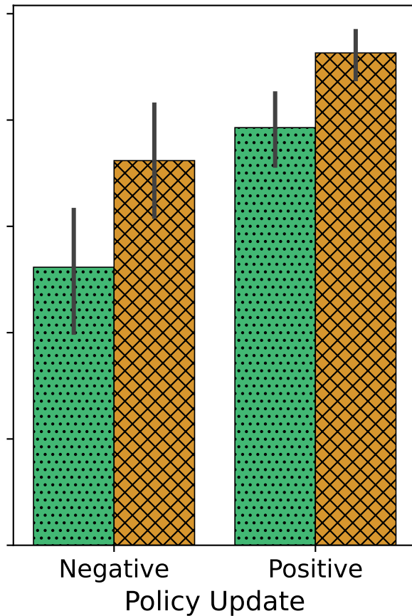
Fruitbot
